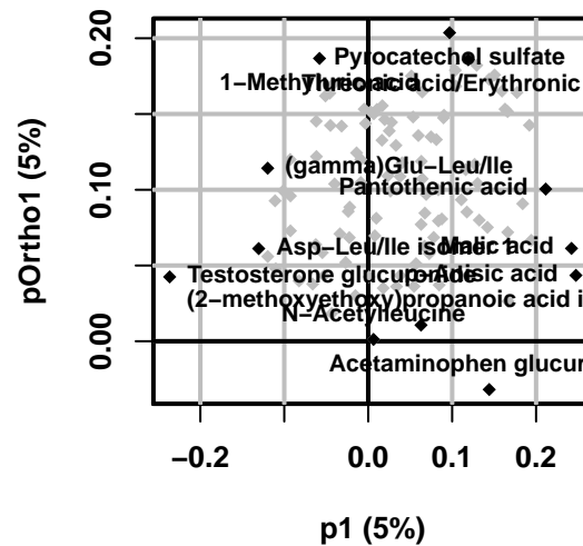
Loadings
