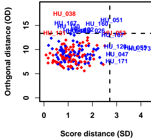
Observation diagnostics
