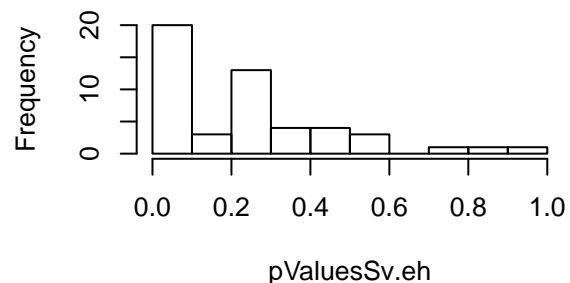
Adjusted p-Values for SVs (Added EH)
